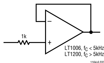
Figure 3. Buffer for Filter Output
