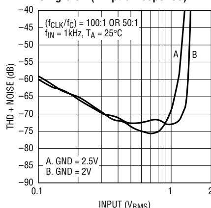
THD + Noise vs RMS Input for Single 5V (Elliptic Response)
